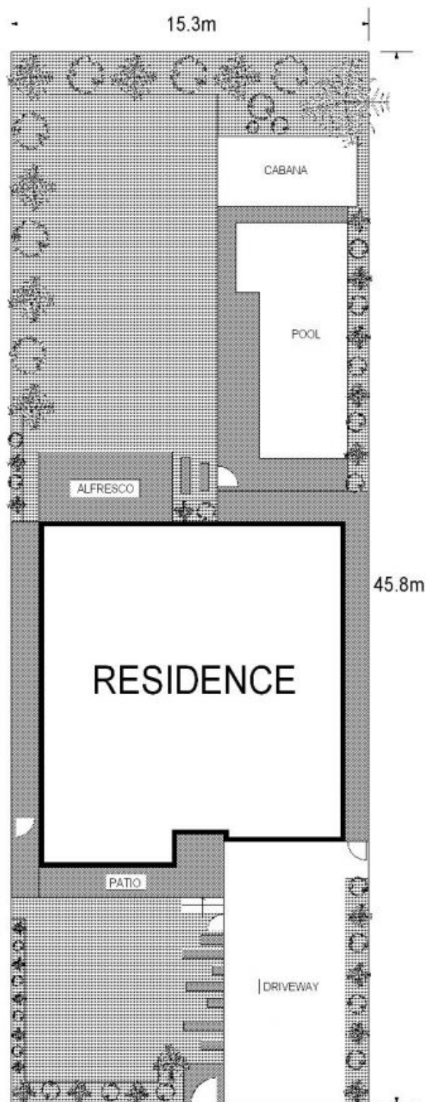
SITE PLAN
