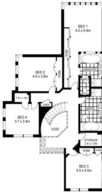
UPPER LEVEL
