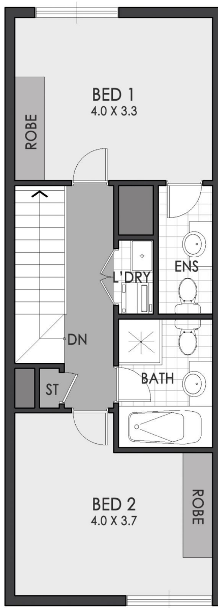
UPPER FLOOR
