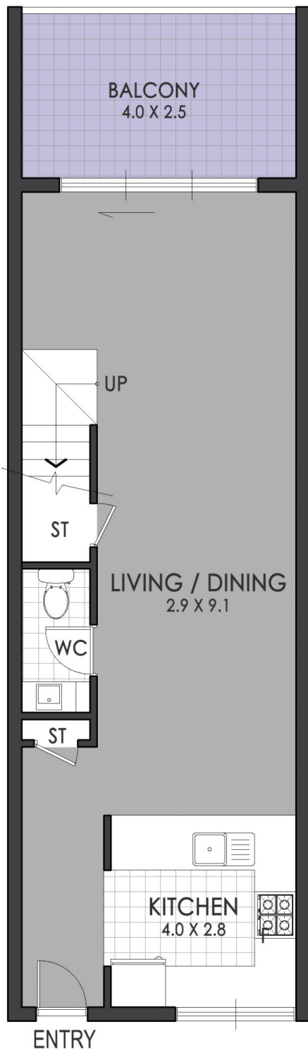
LOWER FLOOR
