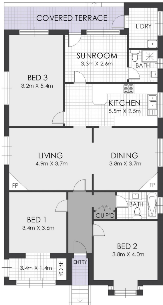
FLOOR PLAN
