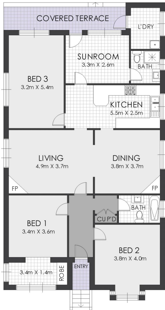
FLOOR PLAN
