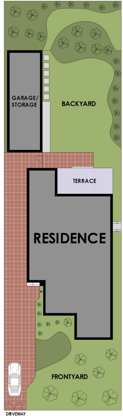
SITE PLAN
